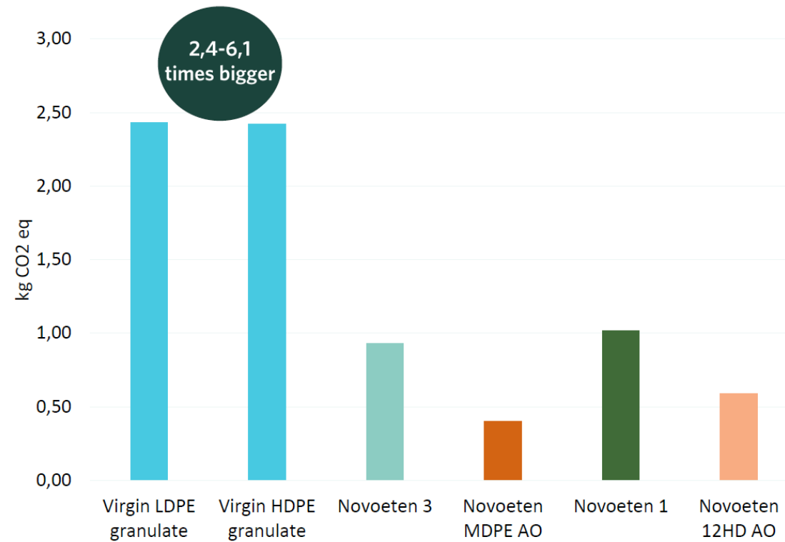
Climate change cradle-to-gate of 1kg different plastic granulates
